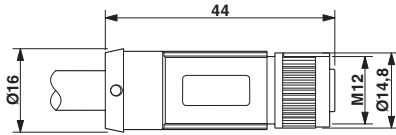
Socket M12-SPEEDCON, straight, shielded
